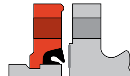
Vic-Flange®
