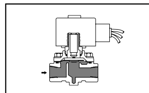
Figure 2B: Pilot Operated, Normally Closed Valve, Energized
