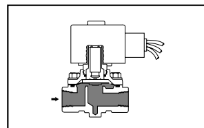
Figure 3B: Pilot Operated, Normally Closed Valve, Energized
