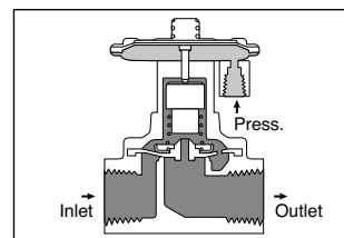
Figure 10B: Normally Closed, Internal, Pilot Operated Valve with Operator Pressurized
